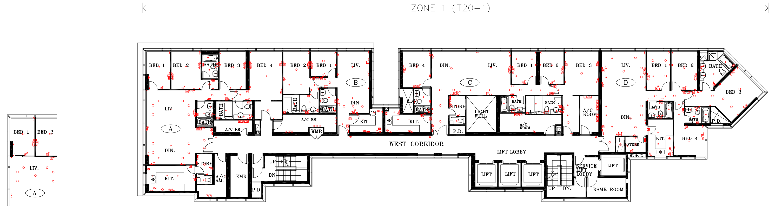
Part Plan of Flat A of 81/F-83/F and 85/F. of Zone 1 of Tower 20* 第20座，第1區，81樓至83樓及85樓A室部分平面圖*
